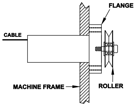
CFF SENSOR
