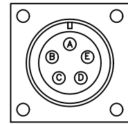
MS3102A14S-5 CONNECTOR
